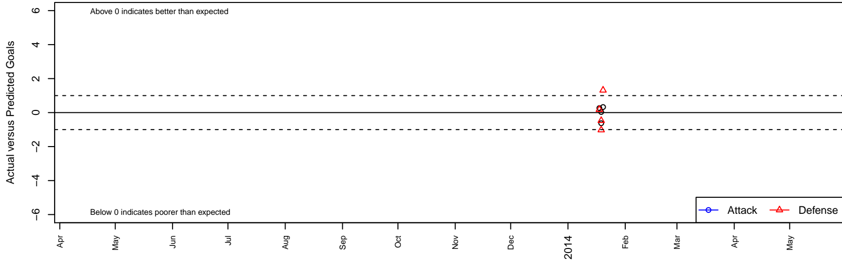
EM Sports Academy B95 Dots are actual minus expected GF (blue circles) and GA (red triangles). Blue line is smoothed change in attack strength. Red is smoothed change in defense strength.
